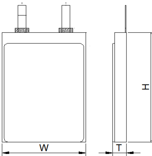
(Maximum) Dimension: T: 6.0, W: 20.0, H: 40.0 Cell (Unit: mm)
